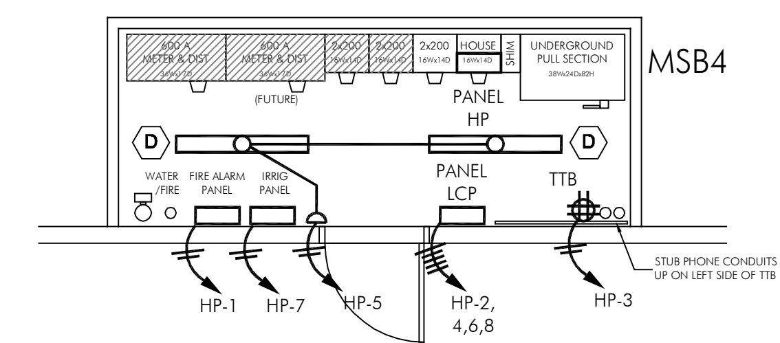
C ELECTRICAL ROOM LAYOUT E4.2 PLAN SCALE: 1/4"=1'
